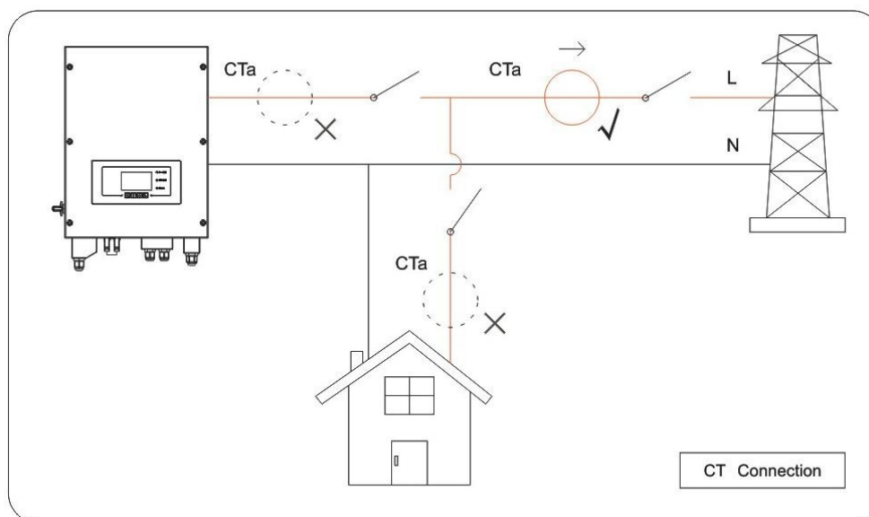
Figure 57 – Raccordements CT
