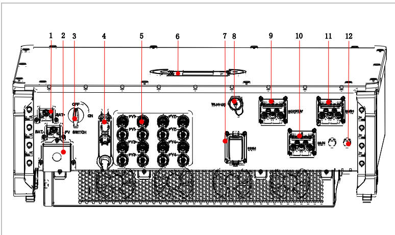
Figura5 -19 Interfaces del AZZURRO 3PH HYD 30000...60000 ZSR
