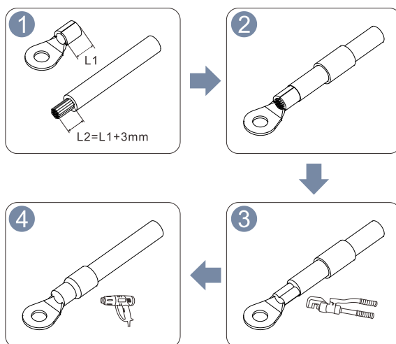
Figure 21 Diagram of Crimping OT terminals
