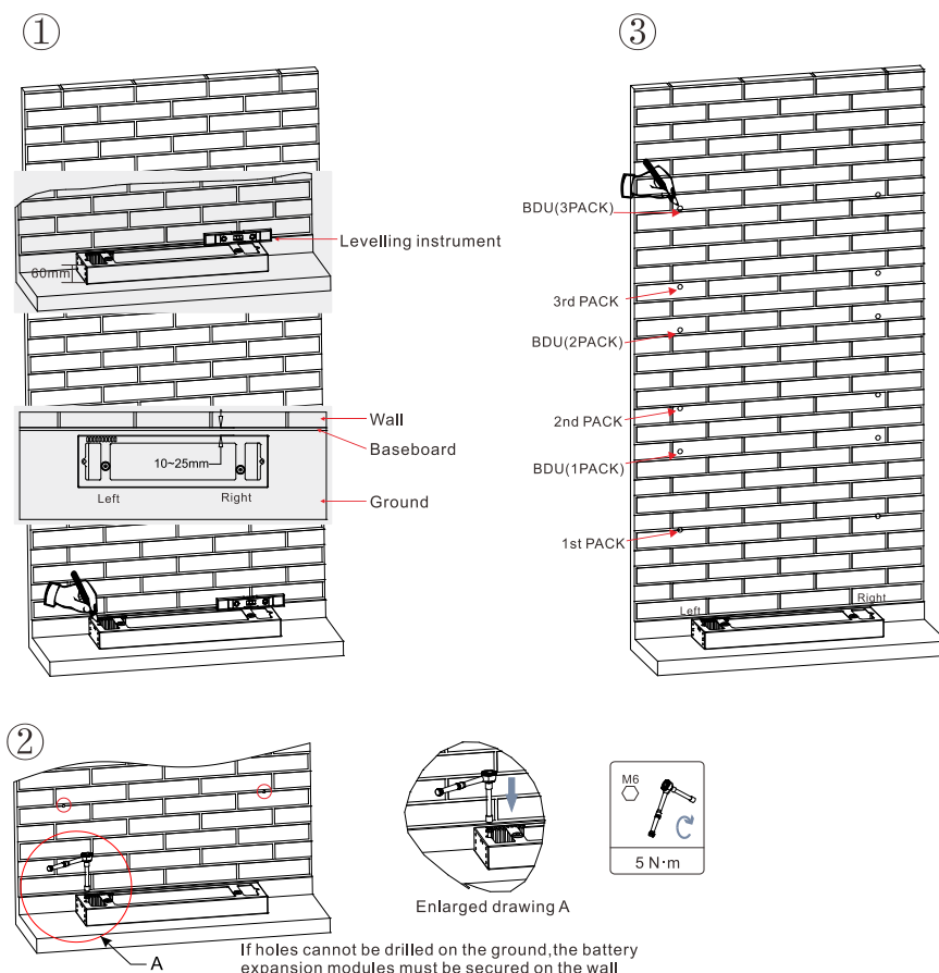
Figure 11 – Base installation diagram
