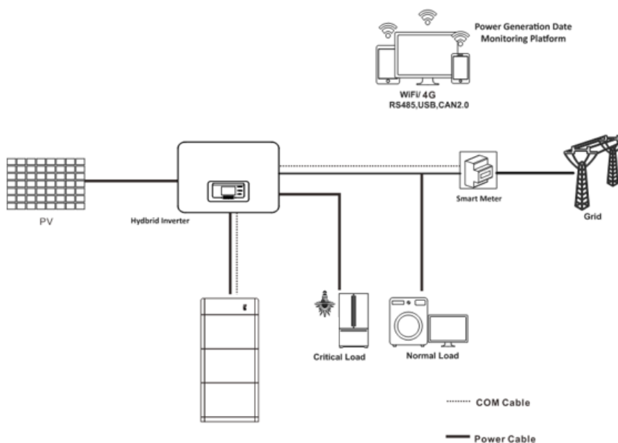
Figure 3 - AZZURRO ZBT-ZBT5K-ES5 ~ ES20 series application principle diagram
