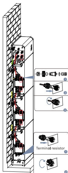
Figure 17 Diagram of internal signal cable connection
