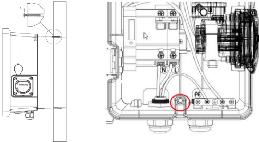
Figure 17 - Wall fixing
