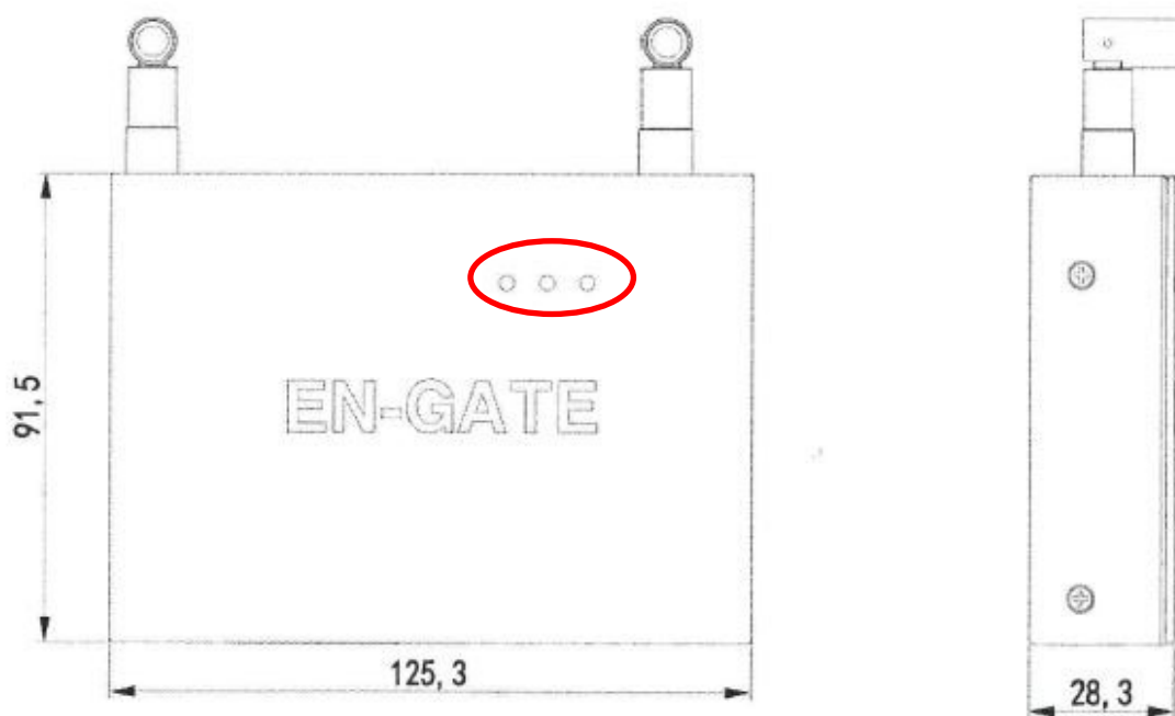
Figure 40 - Device dimensions
