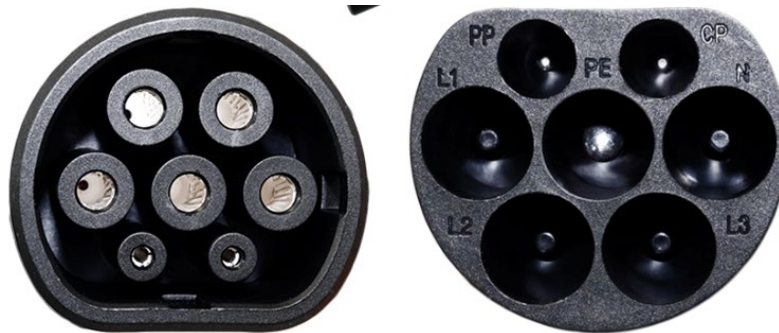
Figura 6 - Conector Type2
