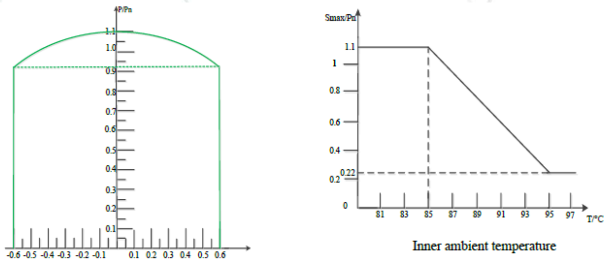
Voltage-dependent PQ diagram for 50KTL-V3
