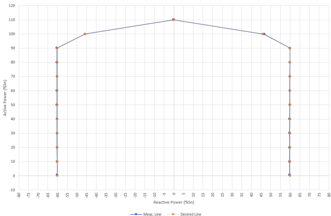
Semicircular Curve (105%Un): Active Power over Reactive Power
