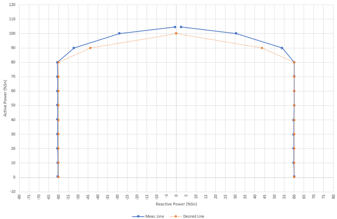
Semicircular Curve (95%Un): Active Power over Reactive Power
