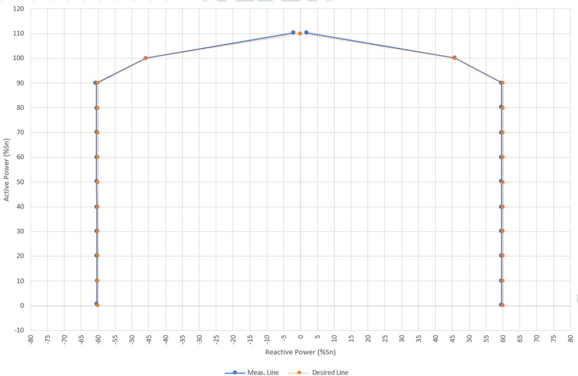
Semicircular Curve (115%Un): Active Power over Reactive Power
