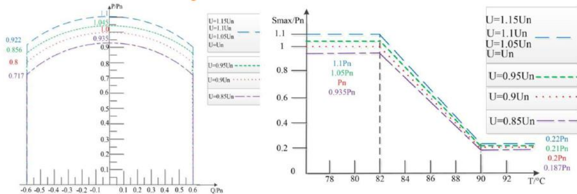
Voltage-dependent PQ diagram for 50KTLX-G3
