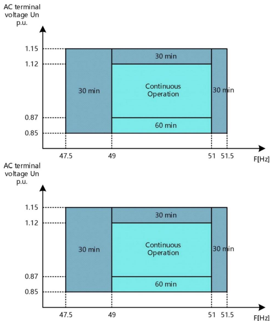
Figure 2 Quasi-stationary operation range for MODEL AZZURRO 3PH HYD 15000~30000 ZSR-L
