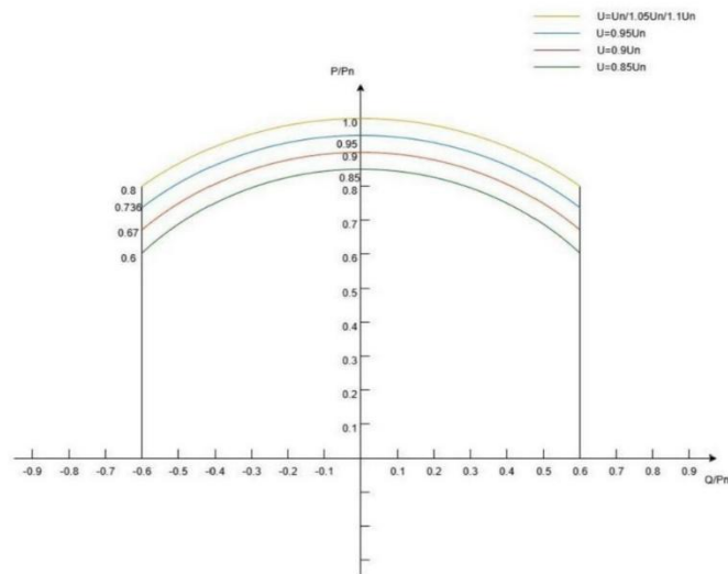
Figure 3 Voltage-dependent PQ diagram for MODEL for MODEL AZZURRO 3PH HYD 15000 ZSR-A-L 、 AZZURRO 3PH HYD 30000 ZSR-A-L
