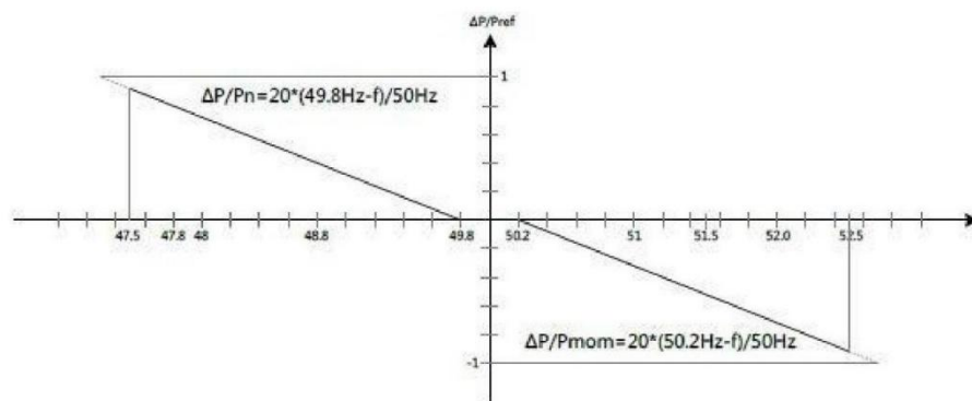
Figure 7 MODEL AZZURRO 3PH HYD 15000~30000 ZSR-L P(f)-diagram
