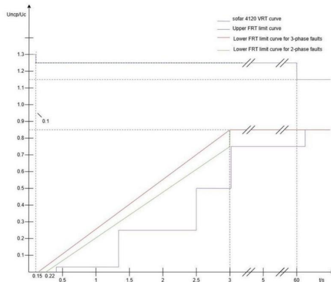
Figure 6 VDE -AR-N 4120 FRT limit curve for MODEL AZZURRO 3PH HYD 15000~30000 ZSR-L
