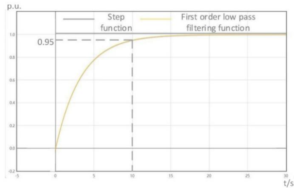
Figure 8 MODEL AZZURRO 3PH HYD 15000~30000 ZSR-L reactive power control feature
