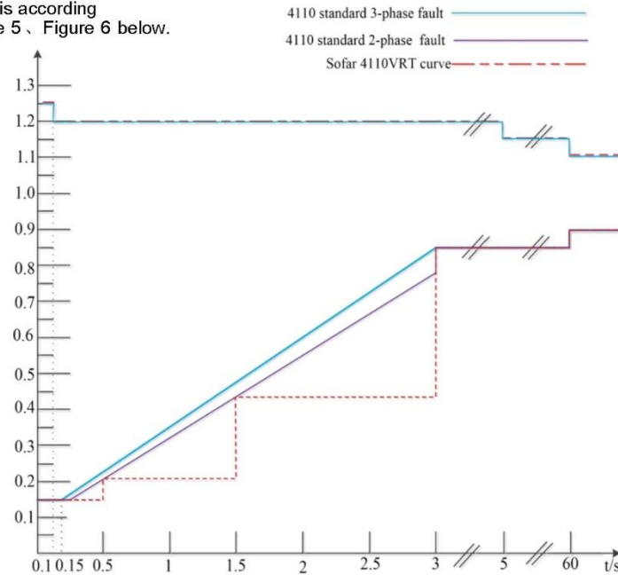
Figure 5 VDE -AR-N 4110 FRT limit curve for MODEL AZZURRO 3PH HYD 15000~30000 ZSR-L
