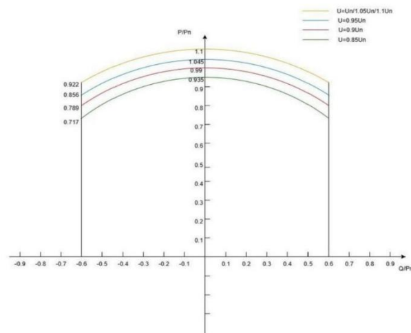
Figure 4 Voltage-dependent PQ diagram for MODEL AZZURRO 3PH HYD 15000 ZSR-L 、 AZZURRO 3PH HYD 20000 ZSR-L 、 AZZURRO 3PH HYD 25000 ZSR-L 、 AZZURRO 3PH HYD 30000 ZSR-L
